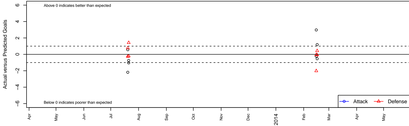
Paso Del Norte Miners B98 Dots are actual minus expected GF (blue circles) and GA (red triangles). Blue line is smoothed change in attack strength. Red is smoothed change in defense strength.
